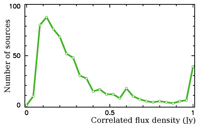
FIG. 2.— Distribution of the correlated flux densities at baseline projection lengths longer than 21.44 megawavelengths. The last bin of the histogram has all the sources with correlated flux density > 1 Jy.
